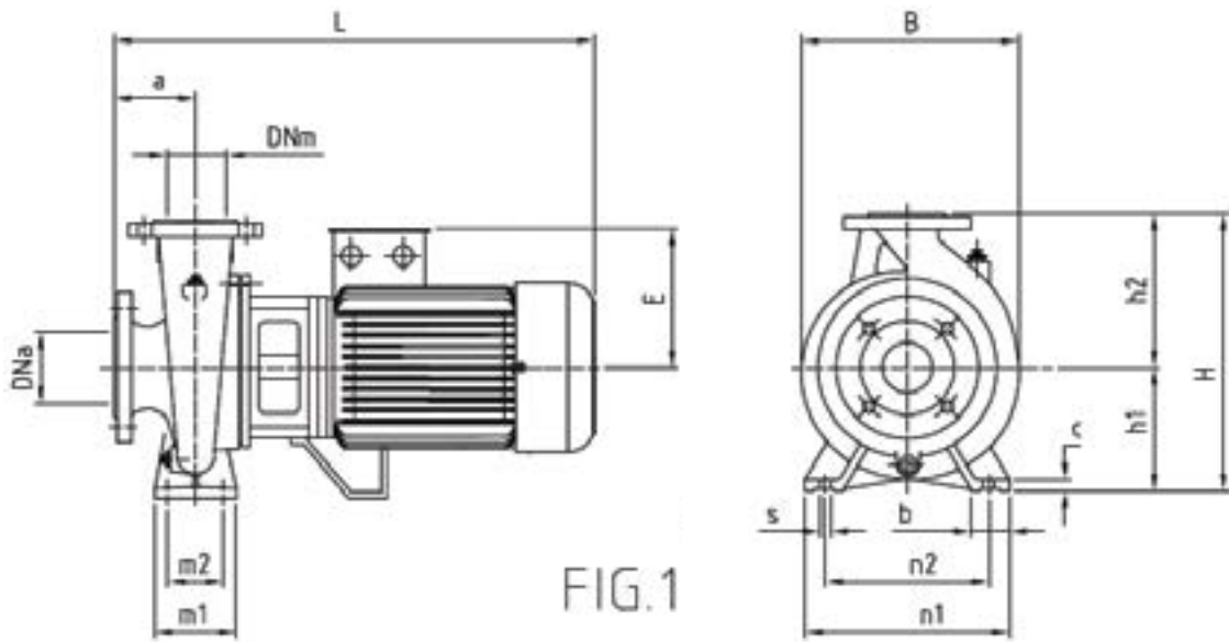
DIMENSIONS [mm]
