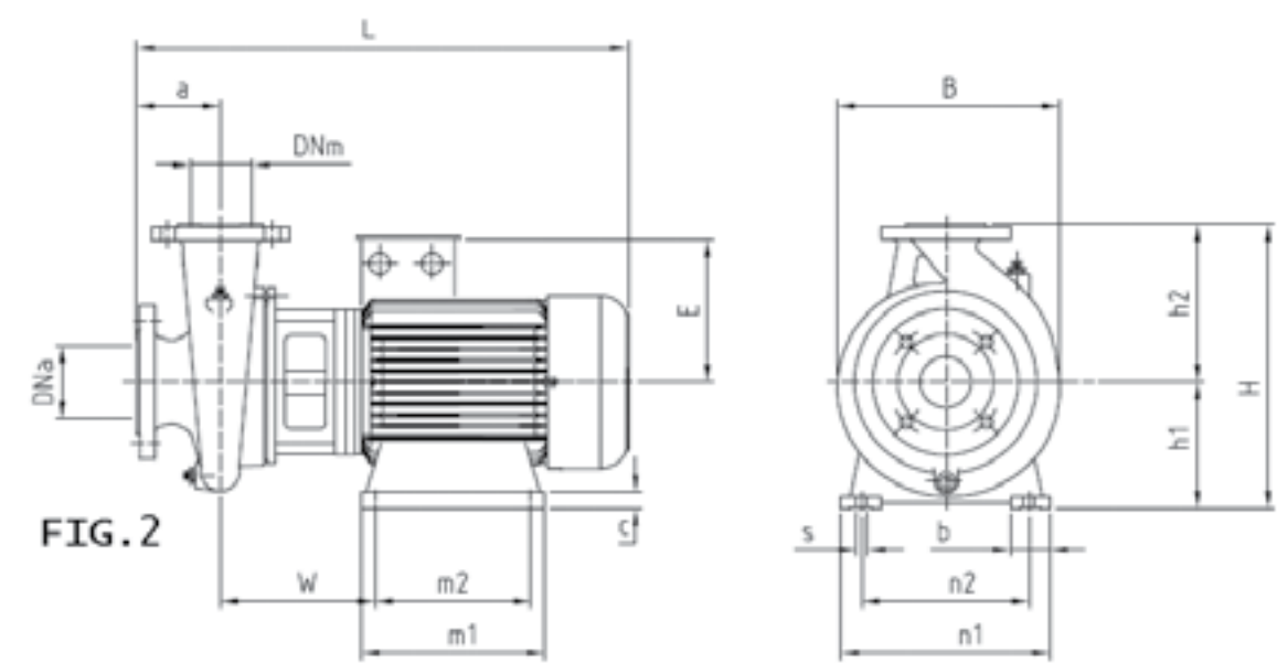
DIMENSIONS [mm]
