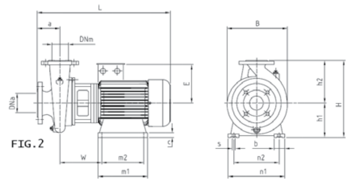
DIMENSIONS [mm]
