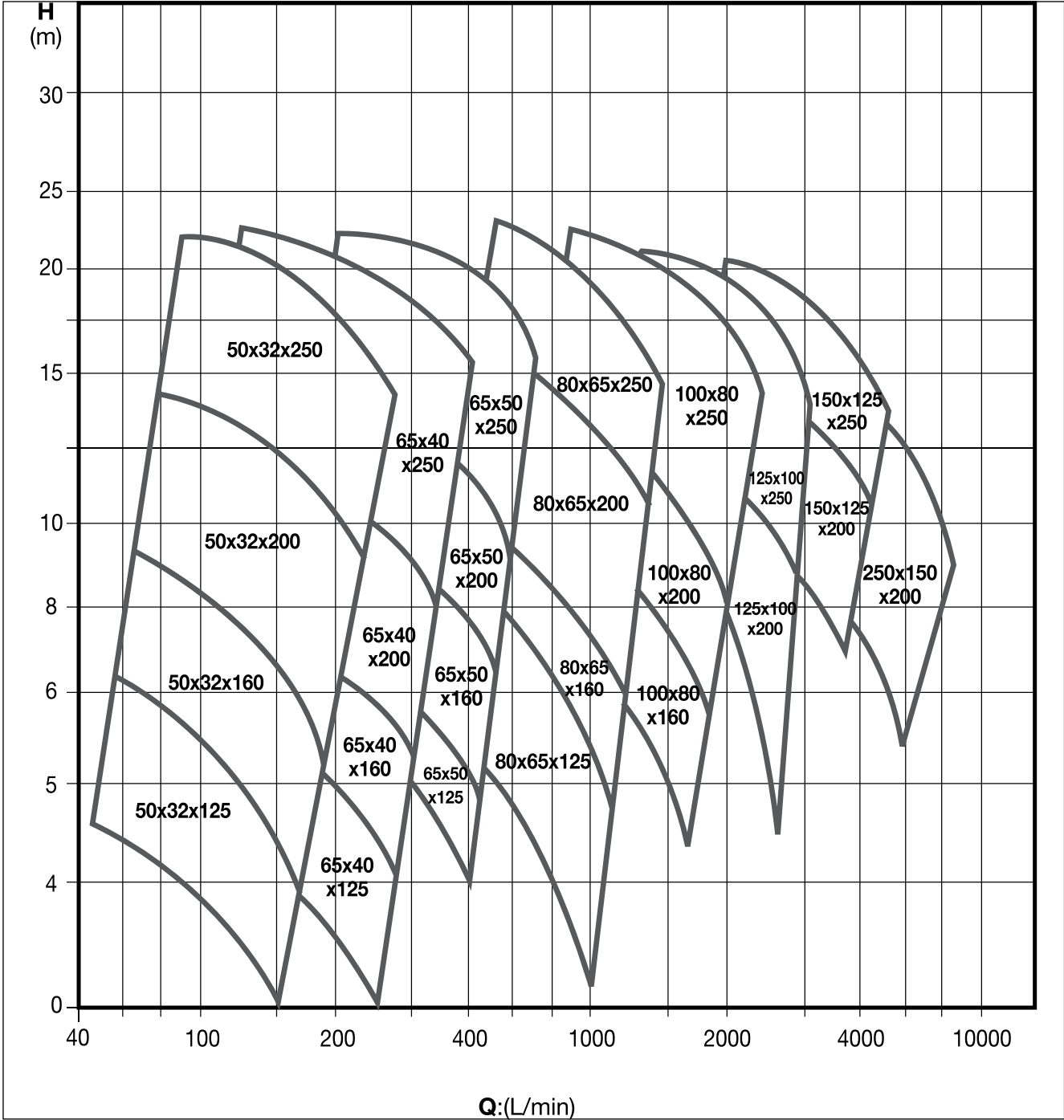
PERFORMANCE
