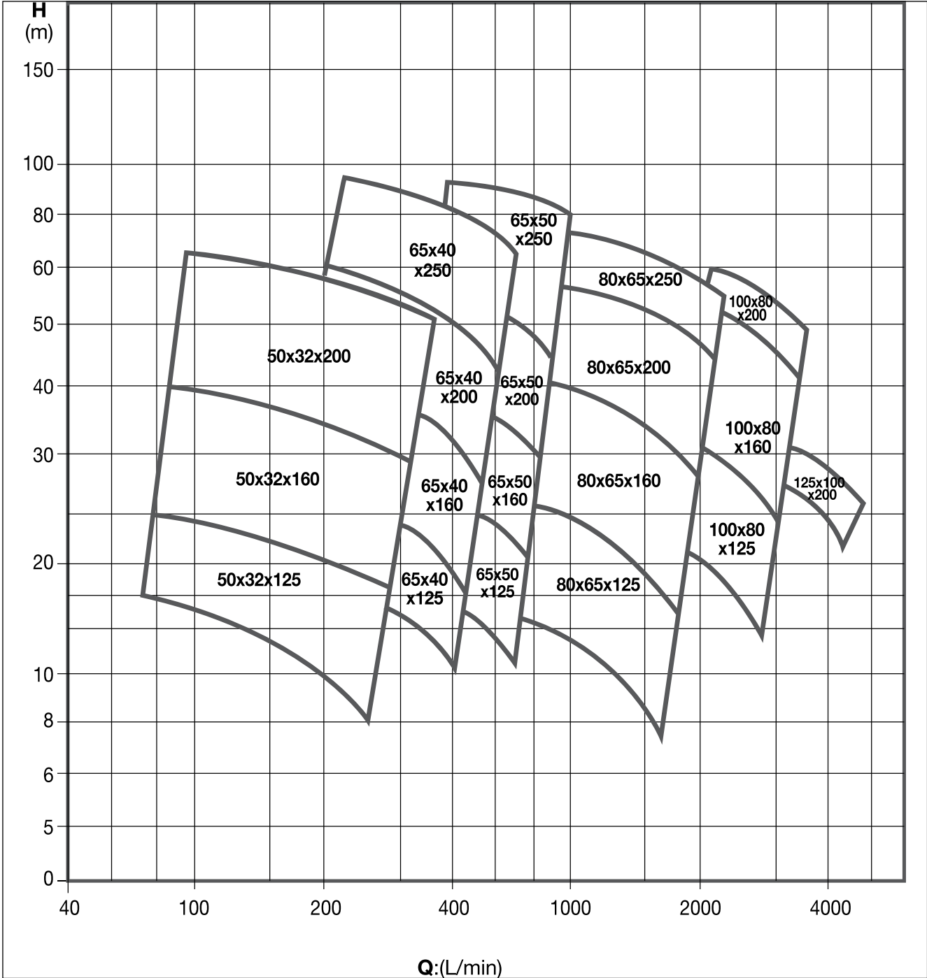
PERFORMANCE
