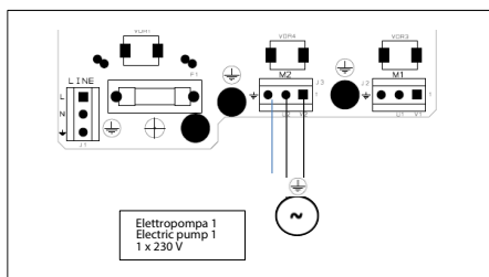
1 electric pump
