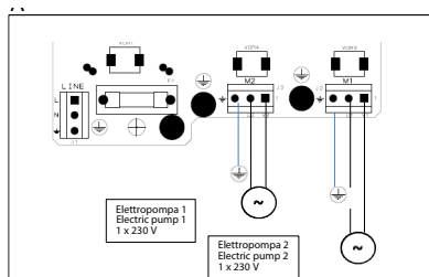
2 electropompe
